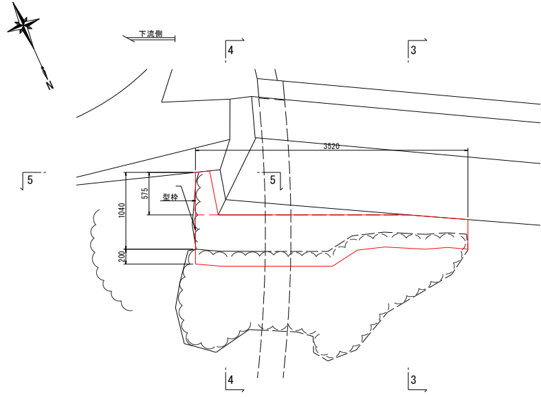
A1橋台基部断面図(3-3)
